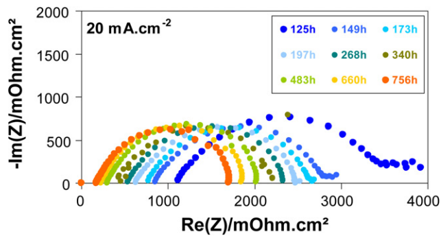
Fig. 10. Evolution of the electrochemical impedance spectra recorded at 20 \text{ mA cm}^{-2} during fuel cell rejuvenation experiment of a Nafion® 212-CS membrane aged ex situ during 258 days at 80^\circ\text{C} and \text{RH}=95\% .
