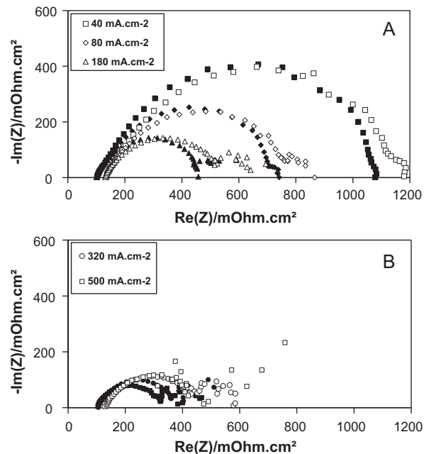
Fig. 12. Electrochemical impedance spectra obtained for MEAs made with a fresh hot pressed Nafion® 212-CS membrane (full symbol) and with a Nafion® 212-CS membrane aged ex situ during 258 days at 80^\circ\text{C} and \text{RH}=95\% after 800 \text{ h} of fuel cell operation (open symbol). (a) 40 , 80 , 180 \text{ mA cm}^{-2} and (b) 320 and 500 \text{ mA cm}^{-2} , 60^\circ\text{C} , 1.5 absolute bars, dry \text{H}_2 at the anode and fully humidified air at the cathode.
